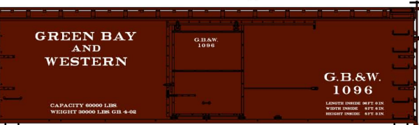
Green Bay & Western 36' Wood Boxcar with Wood Ends & Straight Underframe
